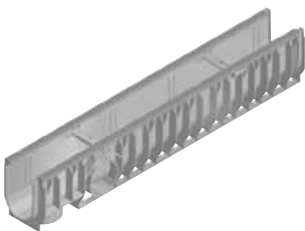
W&H - RECYFIX sportgoot (NW 100 mm), type 010, recht, L x B x H 1000 x 160 x 180 mm, 3,0 kg. Art. nr. WH7600
