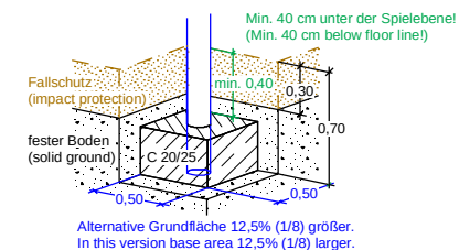
Alternativ: Fundament flach/kantig (Alternative: Foundations plain/edged)
