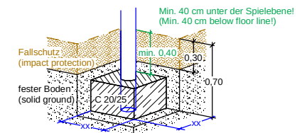
Alternativ: Fundament flach/kantig (Alternative: Foundations plain/edged)
