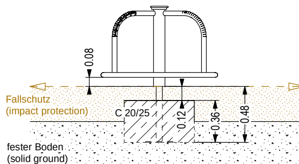
Fertigfundament (Prefabricated foundation)
