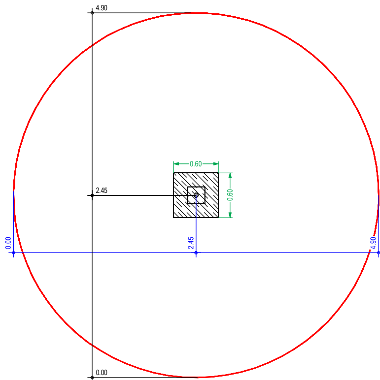
Fertigfundament (Prefabricated foundation)
