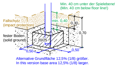
Alternativ: Fundament flach/kantig (Alternative: Foundations plain/edged)
