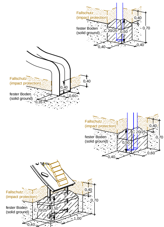
Alternativ: Fundament flach/kantig (Alternative: Foundations plain/edged)
