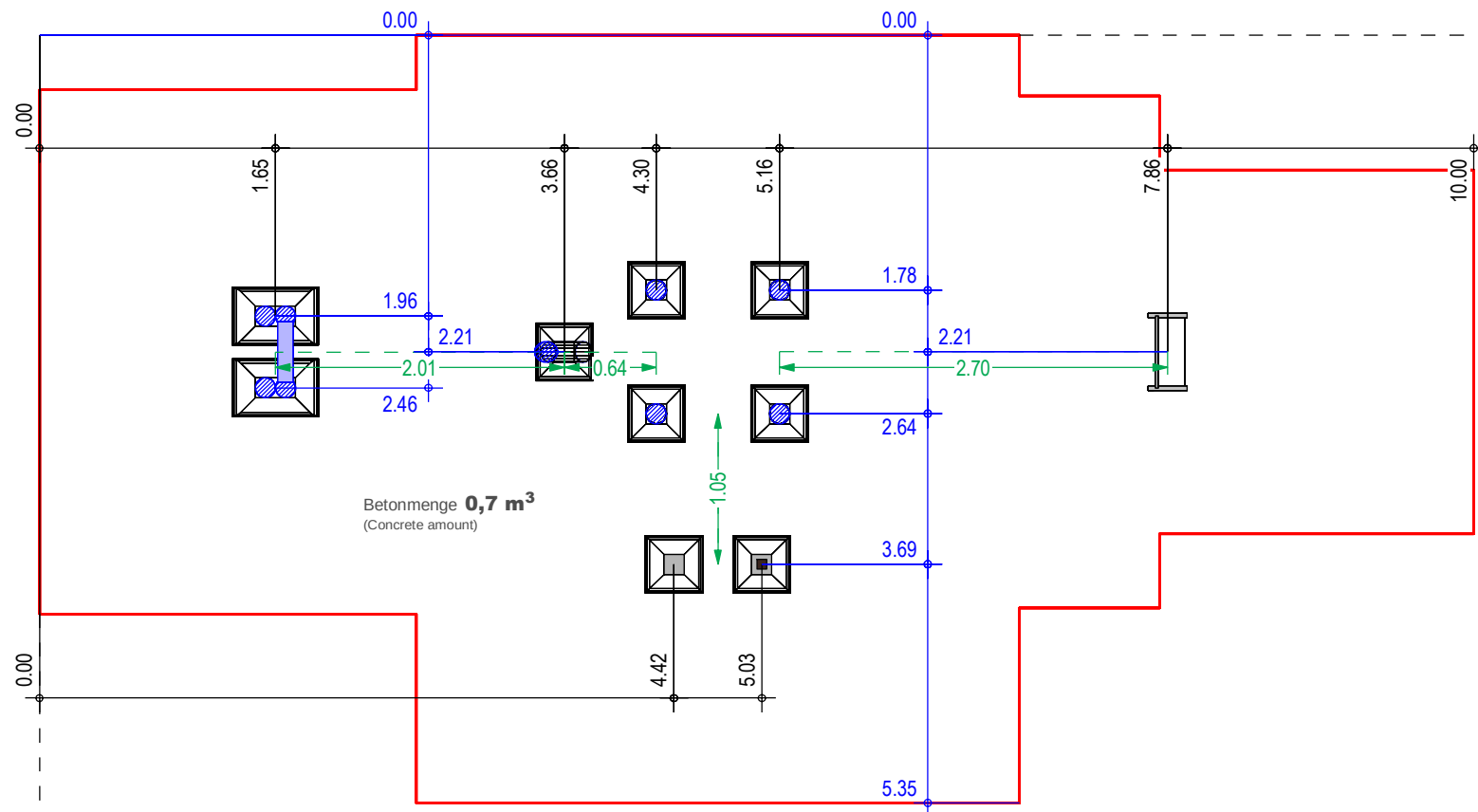
Alternativ: Fundament flach/kantig (Alternative: Foundations plain/edged)
