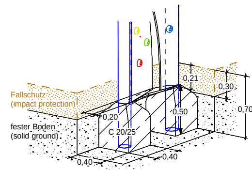
Alternativ: Fundament flach/kantig (Alternative: Foundations plain/edged)
