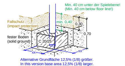
Alternativ: Fundament flach/kantig (Alternative: Foundations plain/edged)
